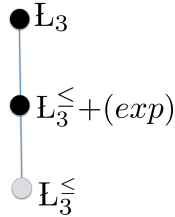
Figure 1: Logics between \mathbf{L}_3^{\leq} and \mathbf{L}_3 in the lattice \mathbf{Int}_{\Pi}(\mathbf{L}_3) .
