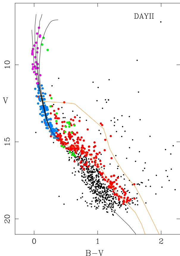
Figure 4. CM diagram V, (B-V) of NGC 3293, showing the photometry by DAYII. The photometric candidate members used to calculate cluster reddening, distance and age are the MS candidate members (blue dots), and post-MS members as magenta dots. PMS candidates are plotted as red dots. Green dots represent stars kept as MS and post-MS candidate members, not used to calculate the cluster parameters. The ZAMS and post-MS isochrones for \text{LogAge}(\text{yr}) = 6.6, 7.0, 7.4 are plotted as black lines. PMS isochrones of ages 1 and 10 Myr are plotted as orange lines. All of them are shifted to account for the mean E(B-V) and DM of the unevolved B-type MS candidate members (see Fig.3), E(B-V)=0.29 , DM=12.02 .
