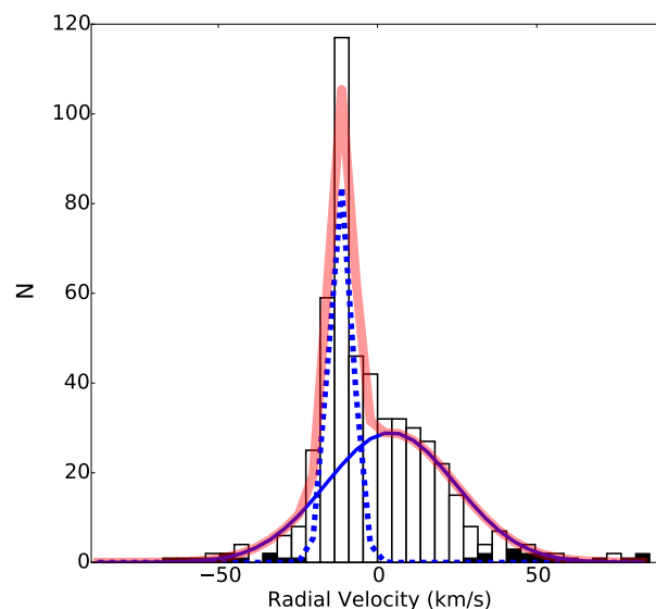
Figure 5. Radial velocity distribution for the 530 stars in the GES data included in our analysis (empty histogram). The filled histogram represents the 28 stars excluded as outliers (see text). The RV distribution is reproduced by the fit of two Gaussian functions: one for field stars (solid blue line) and another for cluster members (dashed blue line), whose sum is overplotted as a solid red line.
