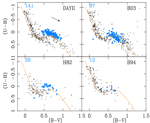
Figure 7. (U - B) , (B - V) diagram by DAYII, B03, H82 and B94. The orange line represents the ZAMS, shifted by values E(B - V)=0.22 , E(U - B)/E(B - V)=0.74 . An arrow shows the direction and length of the reddening vector in the upper left panel. Blue points denote the UF stars in common. Their respective numbers are quoted in each panel.
