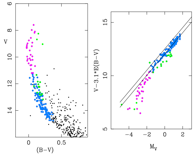
Figure 3. In the right panel the quantity V - 3.1 \times E(B-V) is plotted versus M_V . Lines correspond to maximum (upper line) and average distance modulus of the B-type unevolved MS members, indicated with blue dots. Magenta dots represent evolved stars, used to calculate cluster age. Joint inspection with the CM diagrams, such as the V, (B-V) diagram shown in the left panel, leads to excluding the candidate member stars plotted as green points from these two samples (See text, Sec. 3.1).
