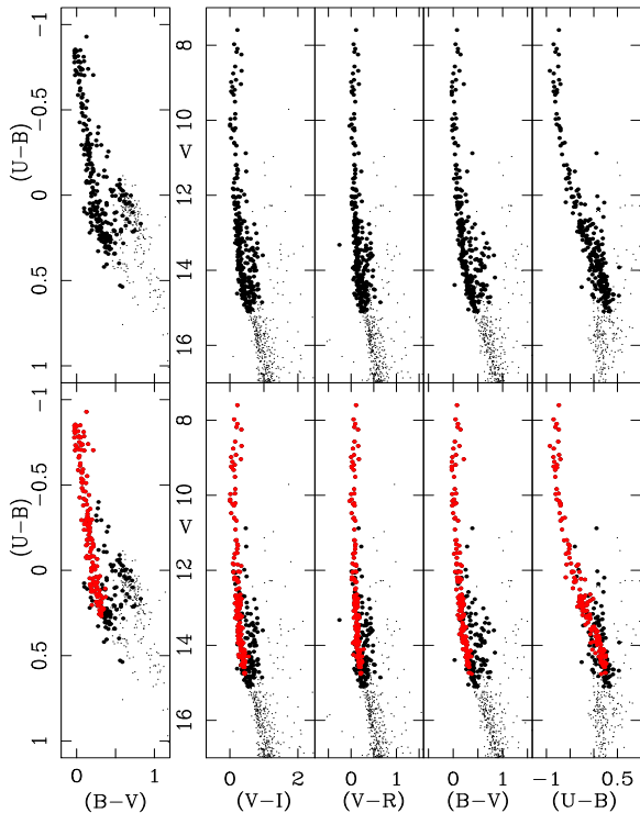
Figure 2. Plots of the (U-B) , (B-V) CC diagram, and the four CM diagrams, V versus colour indices (V-I) , (V-R) , (B-V) and (U-B) , in five panels from left to right. In the upper row, larger dots represent possible stars defining the expected main sequence and evolved stars in each diagram. In the lower row, larger dots represent stars selected in this way in at least one of the five diagrams, while red dots represent those stars selected in all five diagrams simultaneously.
