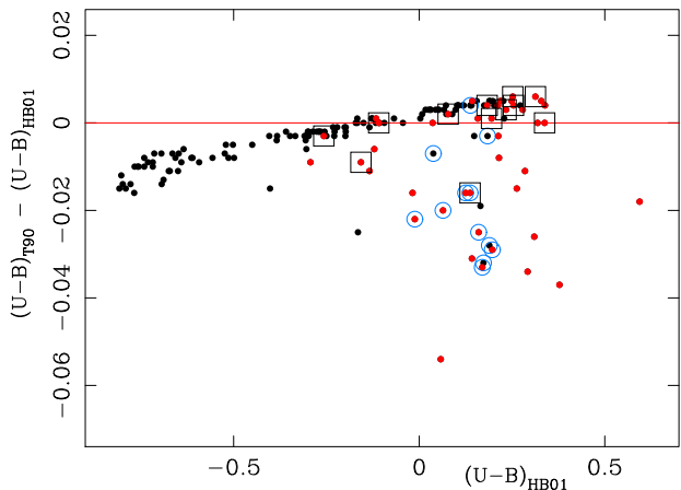
Figure 12. Comparison between (U - B) indices obtained from B94 ubvy photometry by calculation with the formulas by T90 and HB01. A red line marks the zero difference. The UF stars in common between DAYII and B94 are marked with blue circles. Photometric and kinematic PMS probable members are marked respectively with red dots and black squares.
