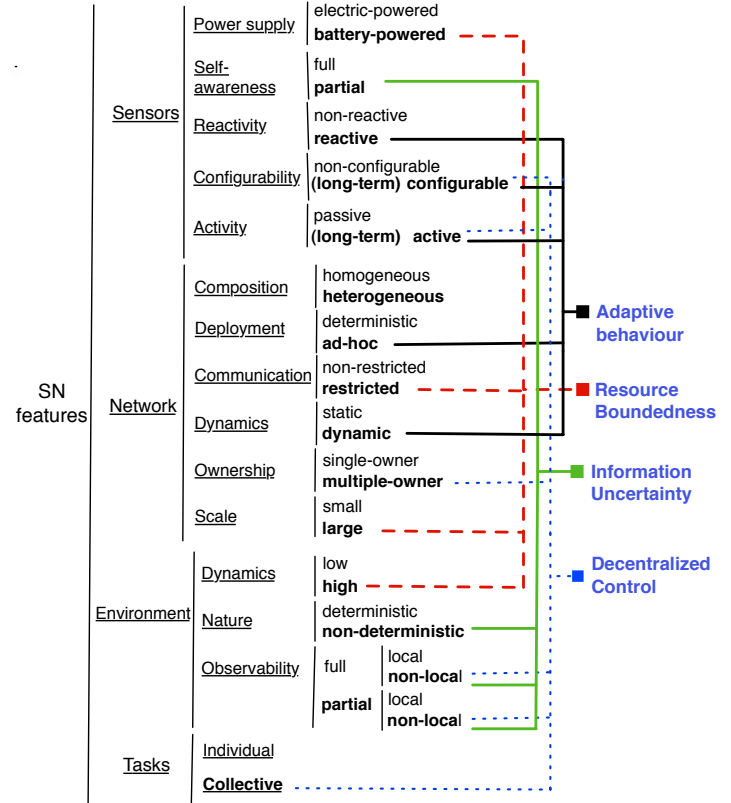
FIGURE 1. A taxonomy for sensor networks.
