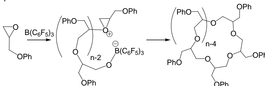
Figure 1. Cyclic poly(glycidyl phenyl ether) obtained by zwitterionic ring-opening polymerization. 1
