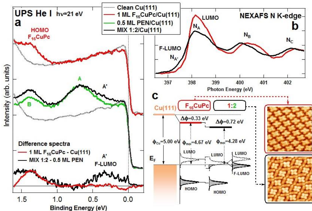
Fig. 3. Controllable charging of F 16 CuPc on Cu(111) by work-function manipulation through its supramolecular environment.
