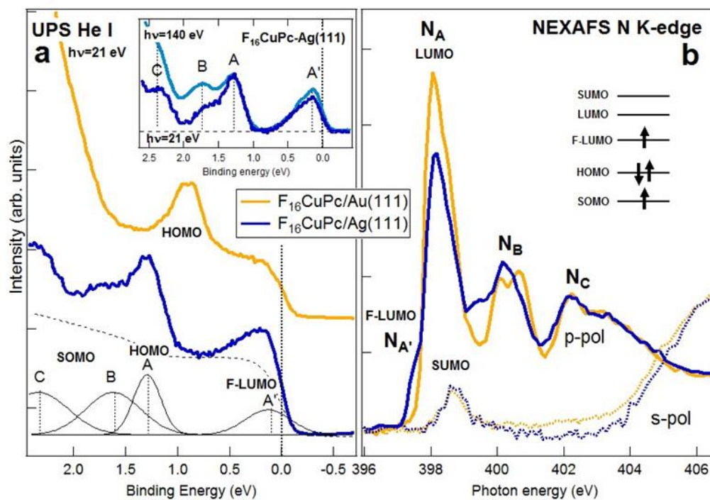
Fig. 2. Analysis of occupied and unoccupied molecular orbitals providing spectroscopic evidence of the partial charge transfer and LUMO level splitting.
