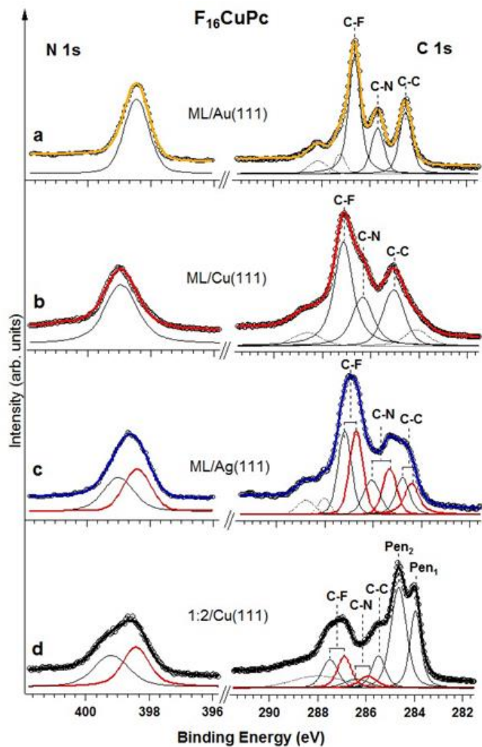
Fig. 4. F_{16}CuPc core level photoemission spectra on varying work-function substrates.
