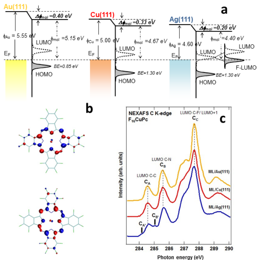
Fig. 1. Interface energetics of F 16 CuPc on coinage metal surfaces of varying work-function, reaching a partial charge transfer scenario with splitting of degenerate LUMO levels.
