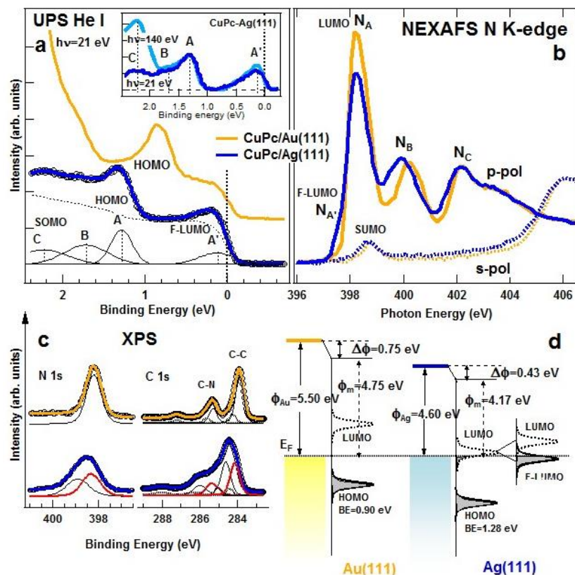
Fig. 5. Comparing the phenomenology for the closely related molecule CuPc.
