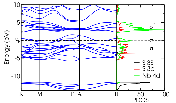
FIG. 5. (Color online) Band structure and projected density of states of \text{NbS}_2 . The zero of the vertical axis indicates the Fermi level.
