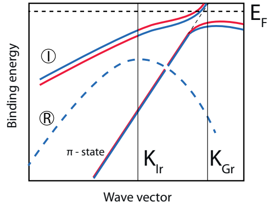
FIG. 4. (Color online) Schematic behavior of the graphene and Pt-Ir interface states near the \bar{K} point of the BZ of graphene.
