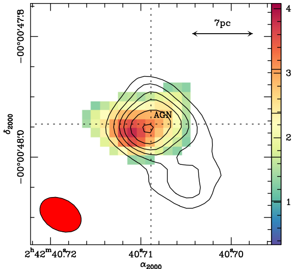
Figure 3. Overlay of the continuum emission contours of Fig. 1 on the CO(6–5) emission (color scale) from the AGN torus. Units are in \text{Jy km s}^{-1} \text{beam}^{-1} .
