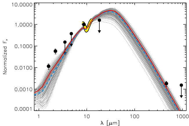
Figure 4. High spatial resolution SED of NGC 1068 (thick yellow line: spectrum; black dots: photometry) normalized to the 8.7\mu\text{m} point. The solid red and dashed blue lines correspond to the maximum-a-posteriori (MAP) and median models respectively for the range 60^\circ < i < 90^\circ . The upper limits correspond to the largest apertures ( \leq 0''.3 ). Grey curves are the CLUMPY models sampled from the posterior distributions compatible with the data at the 68% confidence level.
