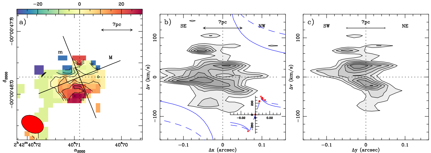
Figure 5. (a) The CO(6–5) mean-velocity map of the torus. The contours span the range ( -30 \text{ km s}^{-1} , 30 \text{ km s}^{-1} ) in steps of 10 \text{ km s}^{-1} . The black lines labeled as M and m show, respectively, the orientations of the major and minor axes of the CO torus ( PA^M = 112^\circ \pm 20^\circ , PA^m = 22^\circ \pm 5^\circ ). (b) The CO(6–5) position-velocity diagram along the M axis. Contours go from 2\sigma to 7\sigma in steps of 1\sigma , where 1\sigma = 4 \text{ mJy}^{-1} \text{ beam}^{-1} . The inset shows the velocities relative to v_{\text{sys}} as a function of radius (in arcseconds) as derived for the H 2 O megamaser spots (red markers) detected along PA^{\text{maser}} = 140^\circ \pm 5^\circ (GR96, GA01). The dashed (solid) blue curve shows the best-fit sub-Keplerian (Keplerian) rotation curve v_{\text{rot}} \propto r^{-\alpha} of GR96 with \alpha = 0.31 (0.50). (c) Same as middle panel but for the m axis. In all panels, velocities refer to v_o(\text{HEL}) = 1136 \text{ km s}^{-1} and (\Delta x, \Delta y) -offsets are relative to the AGN position.
