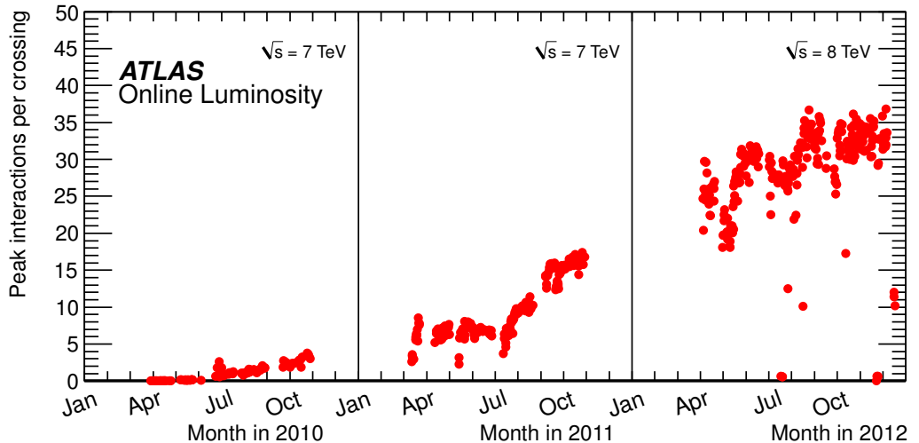
Figure 5.1: The maximum mean number of events per beam crossing versus day during the pp runs of 2010, 2011 and 2012. This figure shows the average value for all bunch crossings in a lumi-block. The online luminosity measurement is used for this calculation. Only the maximum value during stable beam periods is shown. Taken from Ref. [29].
