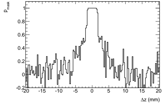
(f) p_{mask} vs. \Delta z , NTrkCut5.
