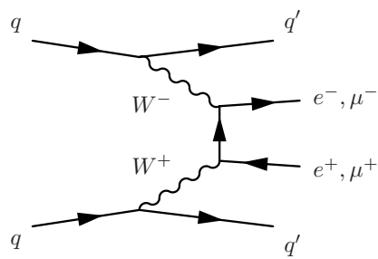
(c) Non-resonant (via W).
