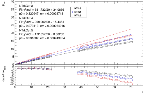
(a) \mu_{rec} vs. \mu , Fitting low \mu
