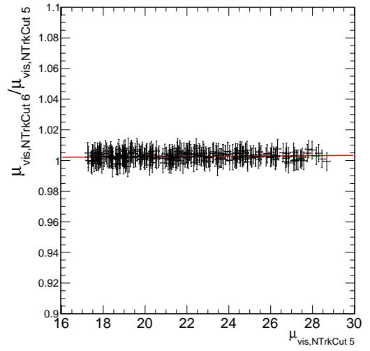
(b) NTrkCut 6 vs NTrkCut 5.
