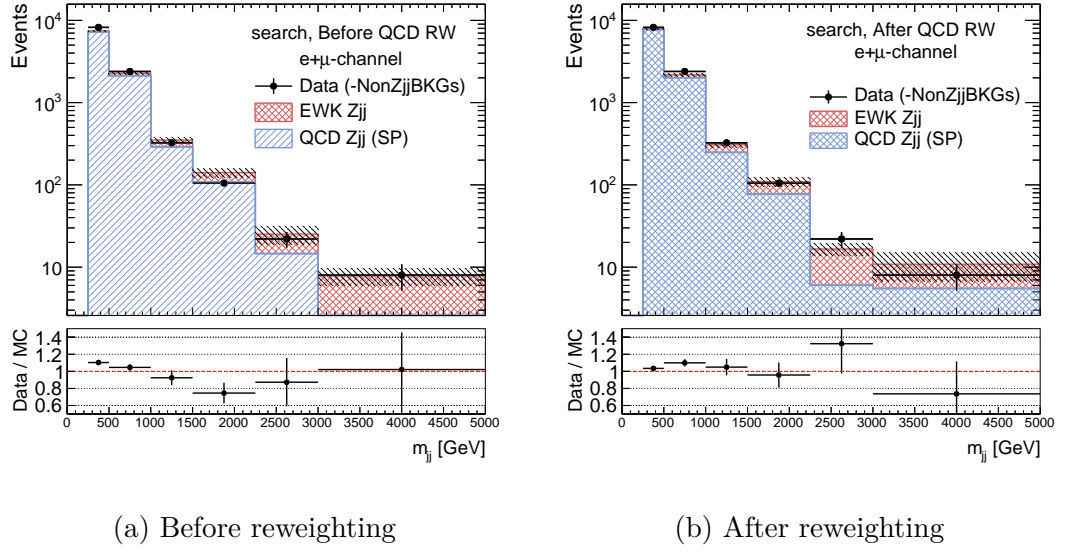
Figure 6.30: Comparison in the search region of the EWK Z_{jj} and QCD Z_{jj} templates to the data (minus the non- Z_{jj} backgrounds) (a) before the reweighting to QCD is applied and (b) after the reweighting is applied, using the QCD Z_{jj} sample form SHERPA.
