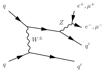
(g) t-channel (via W) and Z.
