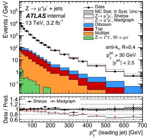
(a) 13 TeV Z +jets analysis.
