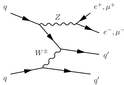
(e) Z and t-channel (via W).
