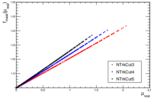
(c) Masking correction.
