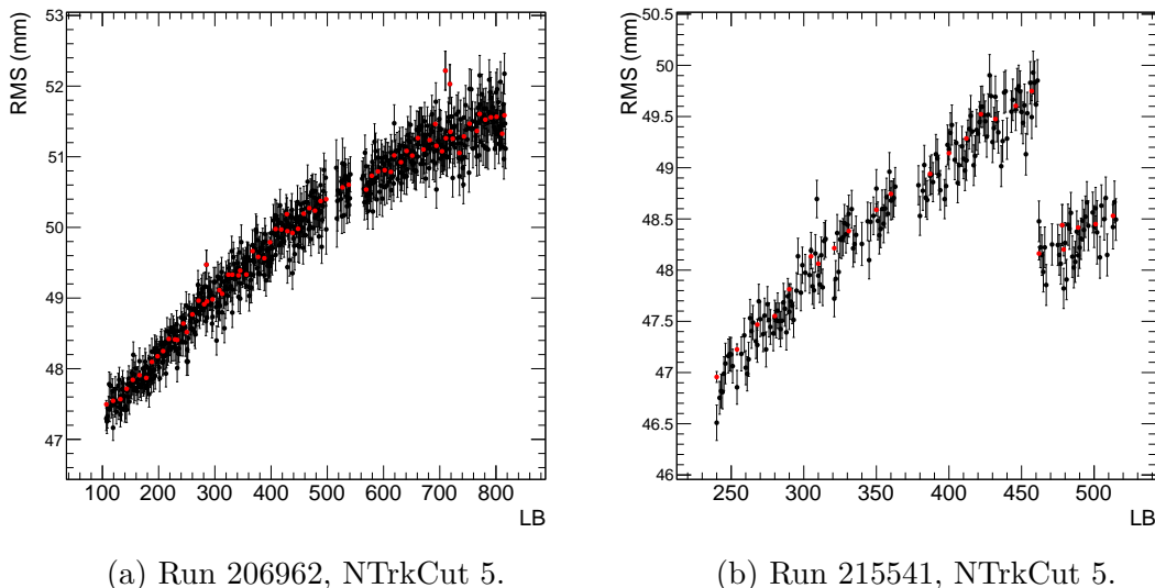
Figure 5.30: Black points correspond to the RMS of z -distribution vs LB for physics runs 206962 and 215541 and NTrkCut 5. Red points correspond to the first LB of the subset of LBs grouped together and the RMS of the z -distribution resulting from grouping those LBs together.
