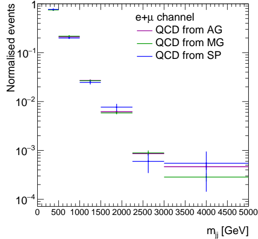
Figure 6.31: Shape comparison of the three available QCD templates after being reweighted using the data/QCD ratios calculated in the control region.
