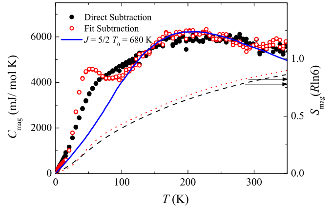
FIG. 7. (Color online) Magnetic contribution to the specific heat ( C_{\text{mag}} ) of \text{CeRuSi}_3 estimated by a direct subtraction of the specific heat of \text{LaRuSi}_3 and of a fit to the \text{LaRuSi}_3 data described in the text. The solid line shows the specific heat of Coqblin-Schrieffer model for J = \frac{5}{2} from Ref. [20], with a characteristic temperature of T_0 = 680 K. The temperature dependence of the entropy in units of R \ln 6 are shown by the dashed and dotted lines for the direct and fit subtractions respectively.
