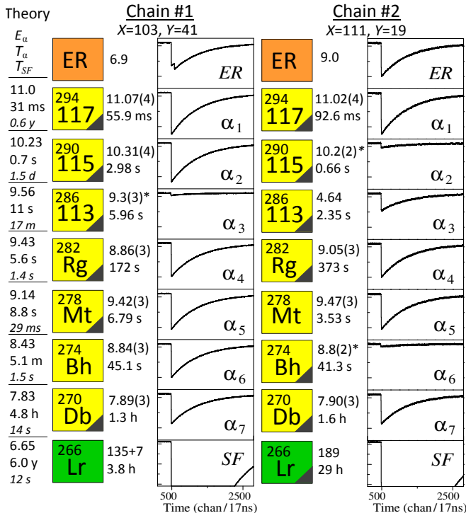
FIG. 1. (Colour online) Decay chains assigned to ^{294}\text{117} . Experimental energies in MeV and \Delta t of all events together with their digitized traces are shown. Energies of reconstructed \alpha particles are marked by an asterisk (*). Boxes with black triangles are corresponding to events observed during beam-off periods. The measured fission fragment energies are from stop+box detectors. Theoretically predicted [38] \alpha -decay energies (in MeV), partial \alpha and unhindered SF half-lives are given on the left.
