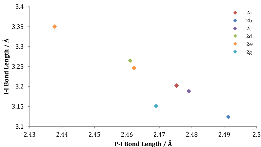
Graph 1: I-I bond lengths vs P-I bond lengths for the donor-functionalised diiodophosphanes. a Compound 2e crystallises with two metrically dissimilar molecules in the asymmetric unit and both are indicated here.
