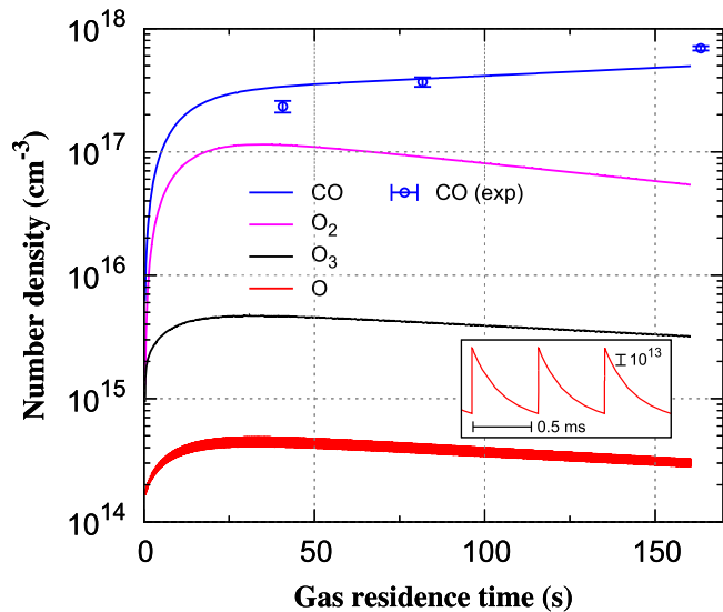
Figure 5. Number densities of the most important species generated by the nanosecond pulsed corona discharge in pure \text{CO}_2 as a function of residence time. Solid lines: numerical simulation. Dots: experimental measurements. The inset shows a magnification of O density (linear scale) around t_g \approx 100 s.
