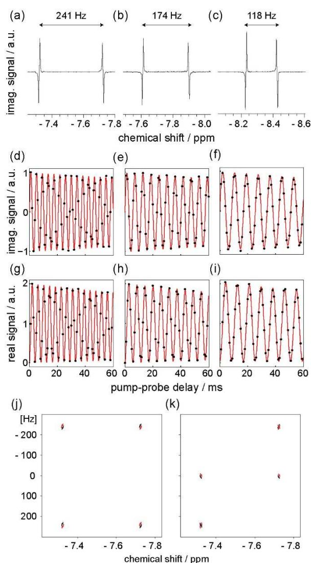
Figure 4. Hydride region of 1D pump-probe ^1\text{H} NMR spectra of 1 in (a) \text{C}_6\text{D}_6 , (b) cyclohexane- \text{d}_{12} , and (c) THF- \text{d}_8 , with \tau = 1 ms and \theta_1 = 90^\circ . Integral of the hydride signals of 1 in the three solvents calculated from pump-probe ^1\text{H} NMR spectra ( \theta_1 = 45^\circ , 0 \leq \tau \leq
