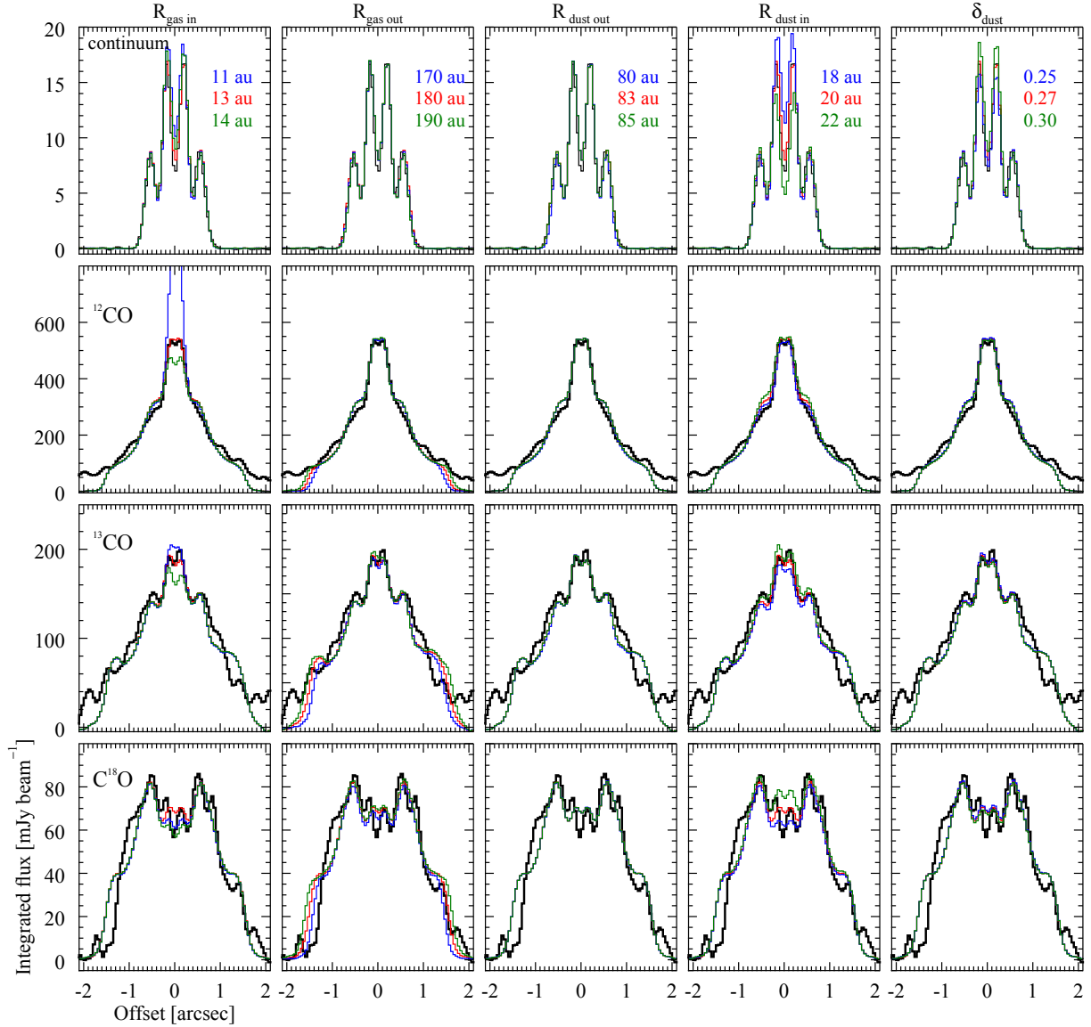
Fig. B.1. Radial intensity profile differences (PA = 5°) for a subset of the model grid. The ^{13}\text{CO} models are scaled up by 10% to match the absolute flux level of the observations.
