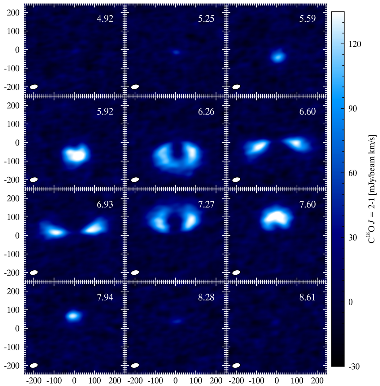
Fig. A.3. ALMA channel maps of C^{18}O J=2-1 .
