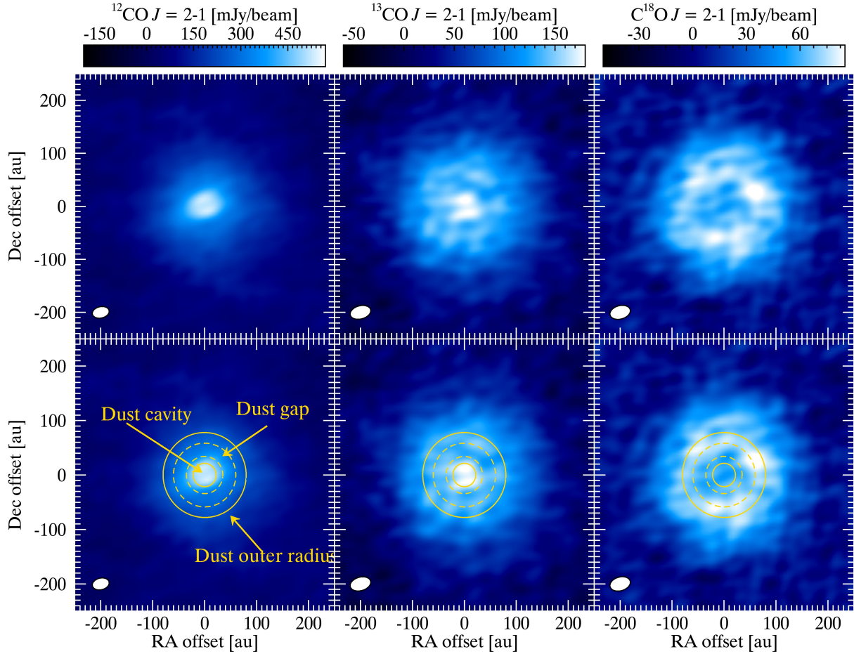
Fig. 2. (Top) Integrated intensity maps (natural weighting) of ^{12}\text{CO} (left), ^{13}\text{CO} (center), and \text{C}^{18}\text{O} (right) J = 2-1 , (bottom) overlaid with the dust rings structure.
