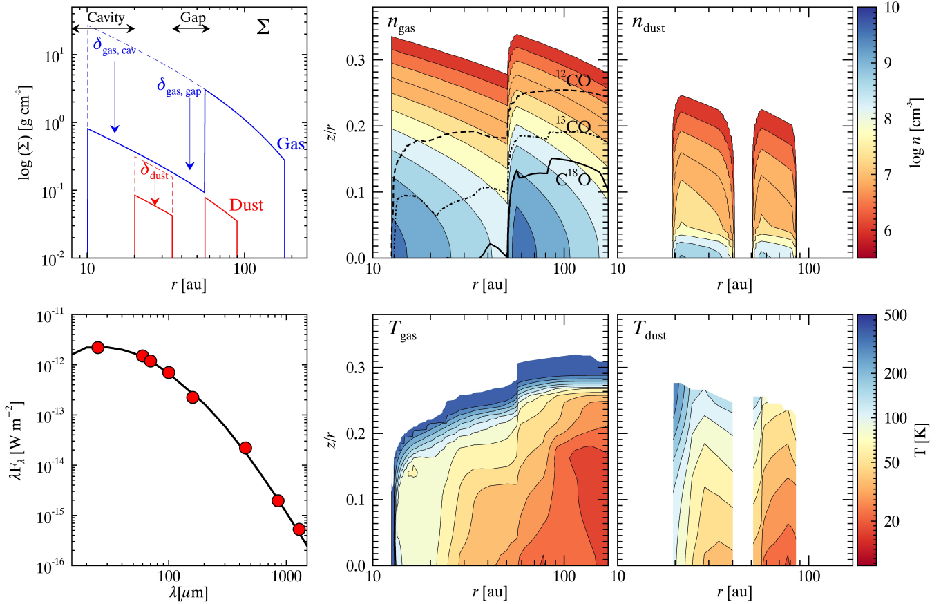
Fig. 5. Fiducial model: ( top left ) surface density profile; ( top middle ) gas density structure: the \tau = 1 layer of the J = 2-1 transition is overlaid as the dashed ( ^{12}\text{CO} ), dot-dashed ( ^{13}\text{CO} ), and solid ( \text{C}^{18}\text{O} ) curve; ( top right ) dust density structure; ( bottom left ) spectral energy distribution with fiducial model (black solid curve): data (red dots) are from IRAS, Herschel (Pascual et al. 2016), SCUBA (Sandell et al. 2011), and ALMA (this work); ( bottom middle ) gas temperature structure; ( bottom right ) dust temperature structure.
