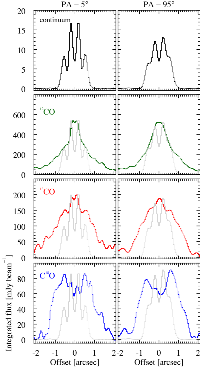
Fig. 3. Intensity profiles of the dust continuum and CO isotopolog integrated emission maps along the major (PA = 5°, left) and minor (PA = 95°, right) disk axis. The normalized continuum profile is overlaid (gray) on the CO panels for comparison. Note that the large-scale (>2'') emission of ^{12}\text{CO} and ^{13}\text{CO} is the result of the reduced image quality (see Sect. 2).
