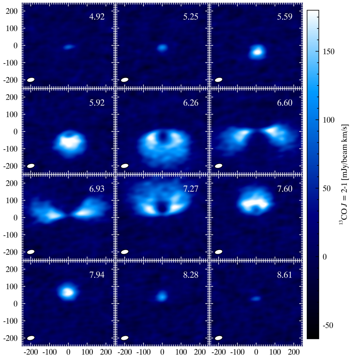
Fig. A.2. ALMA channel maps of ^{13}\text{CO } J = 2-1 .
