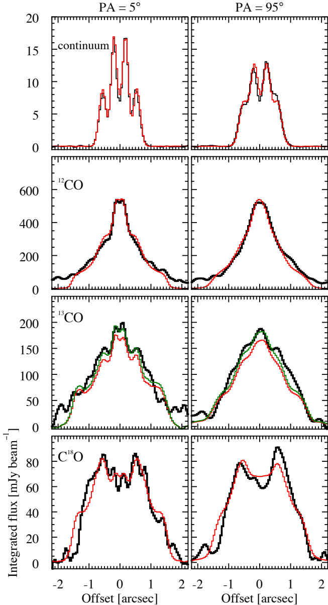
Fig. 7. Results of the fiducial model: comparison of the observed (black curve) and modeled (red curve) radial intensity profiles. In the case of 13 CO, the green curve represents the fiducial model scaled up by 10% to match the absolute flux level.
