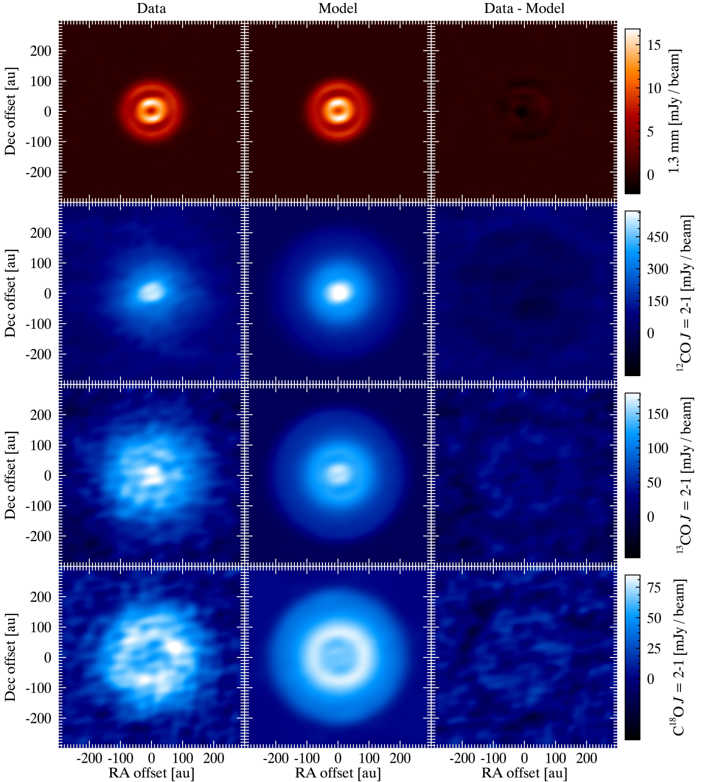
Fig. 6. Results of the fiducial model: (from left to right) ALMA image, model image, residual. Weighting scheme as in Figs. 1 and 2.
