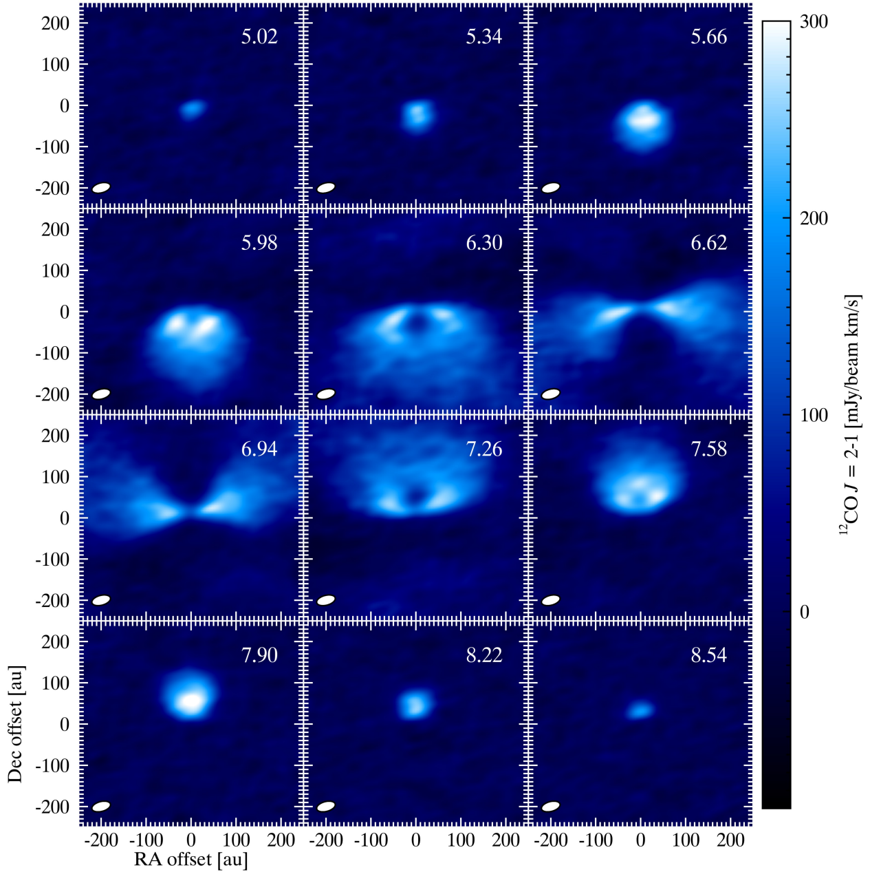
Fig. A.1. ALMA channel maps of ^{12}\text{CO } J = 2-1 .
