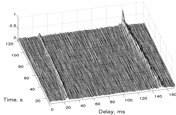
Fig. 14. Fluctuations of the channel impulse response at the first hydrophone in the sea experiment at the distance 46 km.
