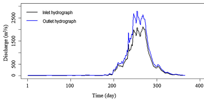
Fig. 4. Simulated hydrographs of the 2007 flood at inlet and outlet of the studied reach (see Fig. 1 for the model domain).
