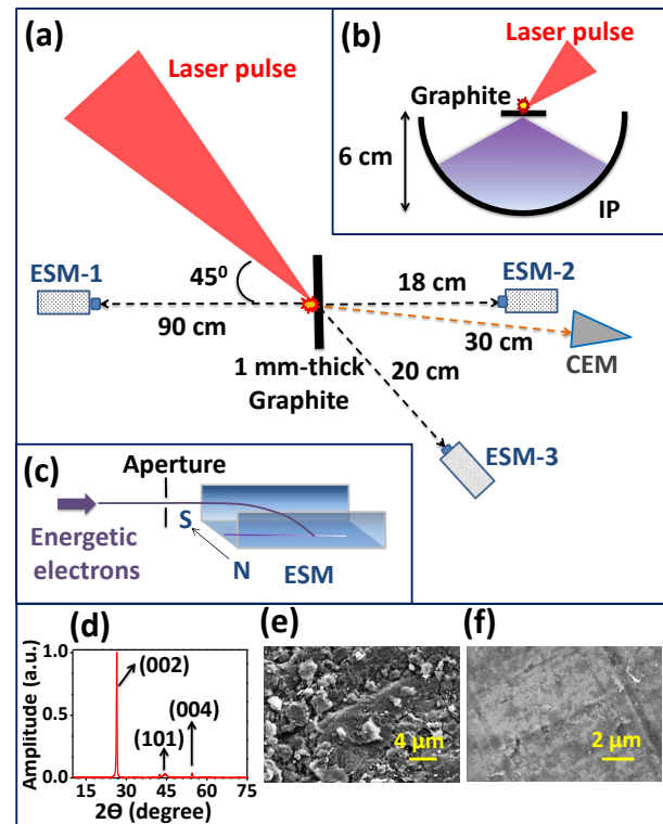
FIG. 1. Experimental setup comprising (a) magnet electron spectrometer (ESM) and channel electron multiplier (CEM) and (b) image plate (IP) covered with 33- \mu\text{m} aluminium foil. (c) Schematic of an ESM. (d) The x-ray diffraction indicates hexagonal structure of the graphite target. The target is polycrystalline in structure. Most of the crystallites (more than 90%) have Bragg planes of type (002), scattering x-rays at an angle of 2\theta = 26.4^\circ . The corresponding inter-planar spacing is 0.337 nm. The average size of these crystallites is 40 nm. (e) and (f) show the scanning electron microscope (SEM) images of the surface structures of graphite and aluminium respectively.
