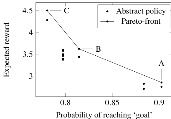
Figure 3: Plot of abstract policies that satisfy the safety constraints C_1 and C_2 , and the Pareto front of safe policies A, B and C.
