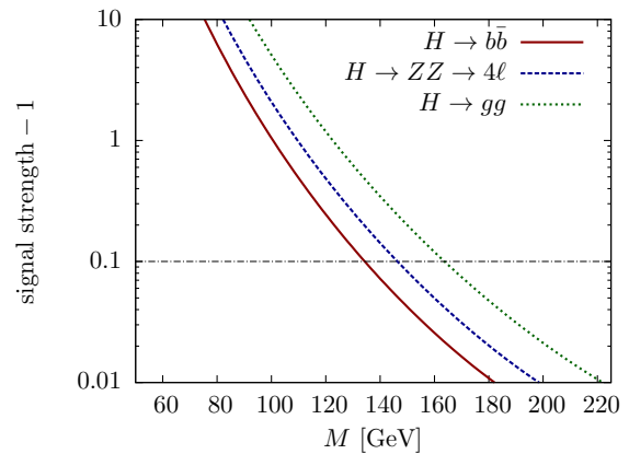
FIG. 5: Modifications of the Higgs boson signal strength as a function of M for the gluon fusion production mode at 8 TeV, estimated using Higgs effective field theory [64–66]. The modifications are analogous to the 2-body and 4-body decay sample Feynman diagrams shown in Fig. 2.
