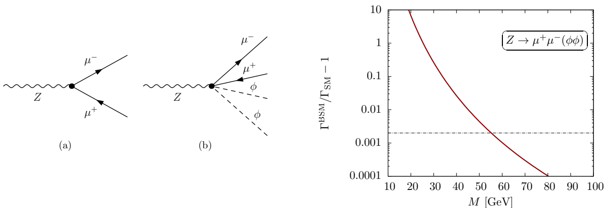
FIG. 2: Modification of the Z boson width to leptons (here concretely for Z \rightarrow \mu^+\mu^- ) due to “dressing” the decay using the new interaction with two scalars. The leading order Feynman diagram contributing to this decay is shown in (a) and an example diagram contributing to the modification of the decay at \sim 1/M^4 is shown in (b). Note that the individual fermion legs and the Z boson propagator can also be dressed with a \phi^2 insertion and these diagrams are not shown. Similarly the production of the Z boson receives modifications. The vertical line represents the current bound on Z \rightarrow \mu^+\mu^- [39].
