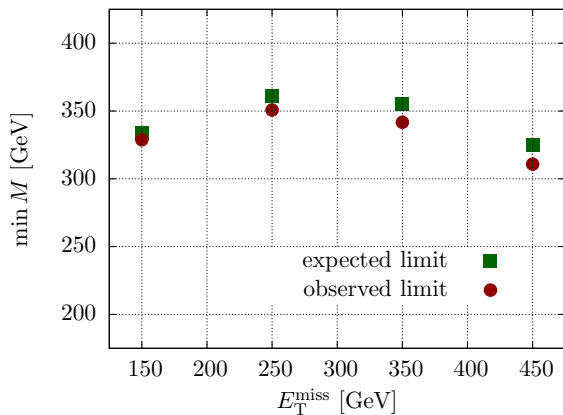
FIG. 3: Results of the ATLAS dilepton search confronted with disformal scalar coupling model. For further details see the text. ATLAS do not quote uncertainties and hence we only show central values.
