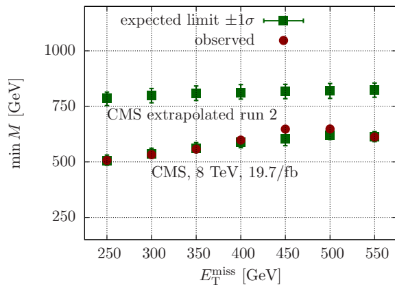
FIG. 4: Minimum scale M extracted from the CMS mono-jet search of [33] in the different search regions based on the inclusive search regions characterised by E_T^{\text{miss}} (for details see text). We also show the improvement based on an extrapolation of the 8 TeV analysis to the 13 TeV LHC run 2 with 100/fb.
