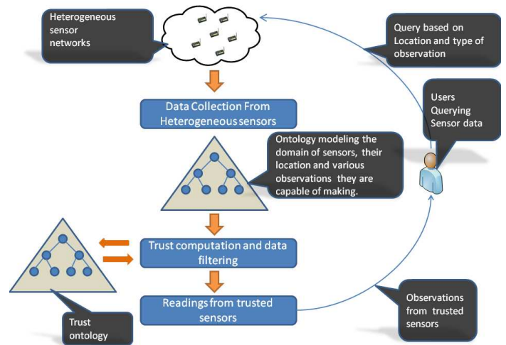
Fig. 2. Trust Ontology applied to Sensor Network scenario.
