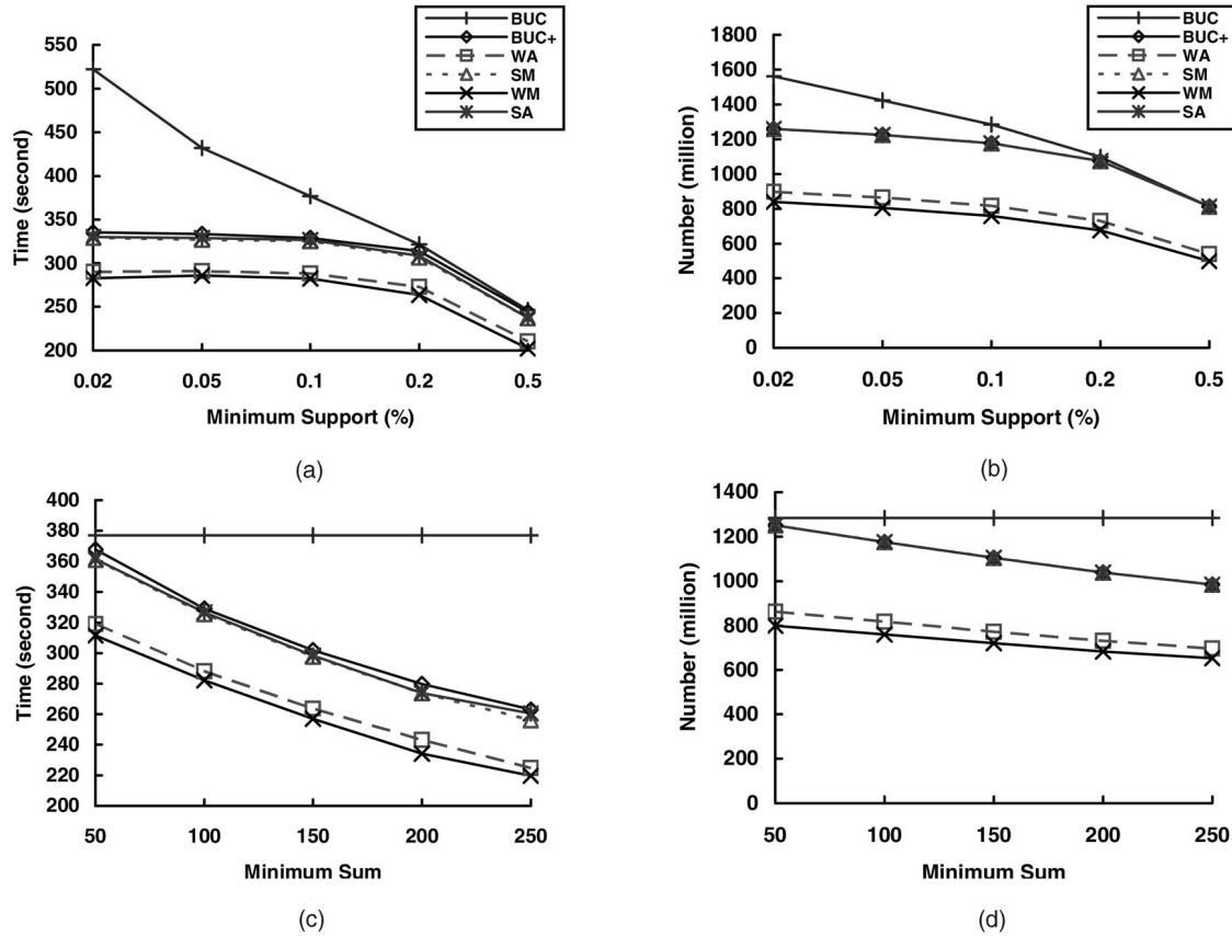
Fig. 7. Experiments on the KDD-CUP-98 data set.
