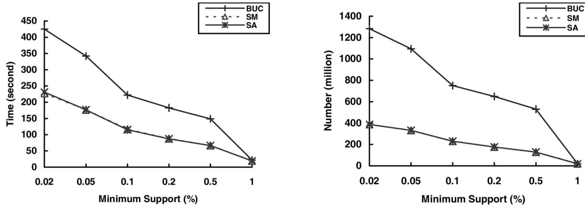
Fig. 3. Minimum support only.
