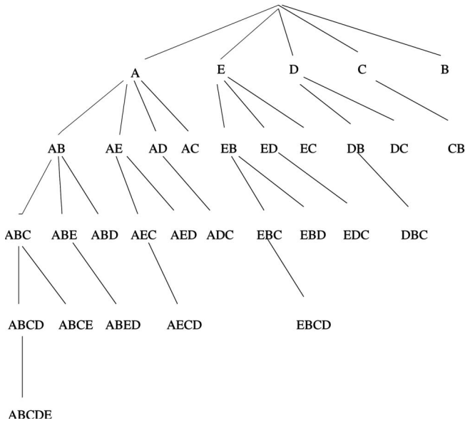
Fig. 2. The rollback tree for A, B, C, D, E .
