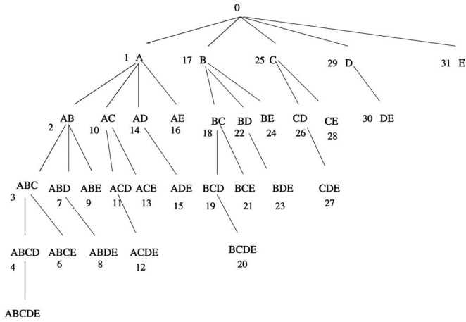
Fig. 1. The lexicographic tree for A, B, C, D, E .
