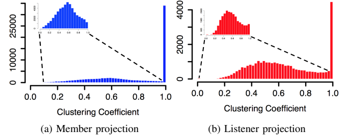
Fig. 7: Projection network cluster coefficient distributions
