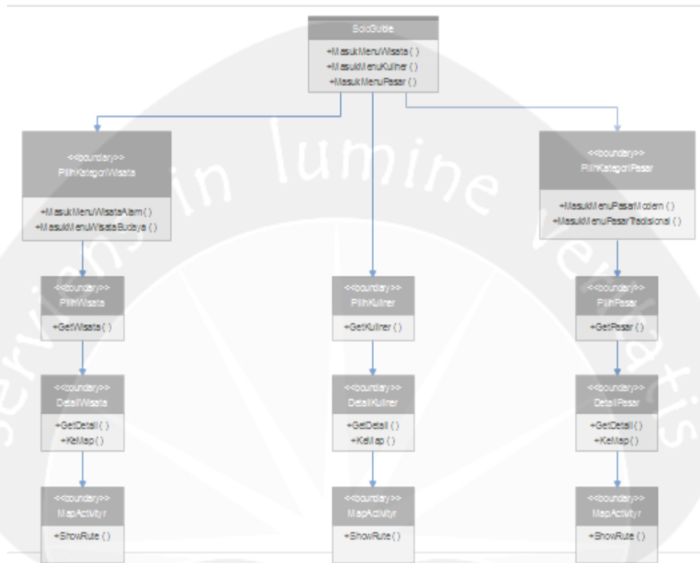
Gambar 2.5. Class Diagram SoloGuideApp
