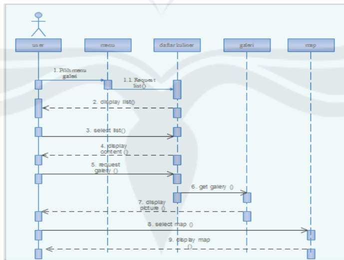
Gambar 2.3. Sequence Diagram : Fungsi Tampil Kuliner
