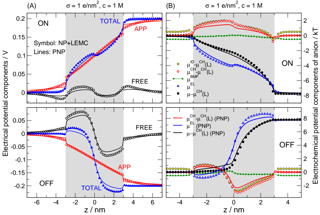
FIG. 8: (A) Electrical potential profiles and components (see Eq. 17) as obtained from NP+LEMC and PNP. Component \Phi^{\text{FREE}}(z) is the product of ions and pore charges in the system, while \Phi^{\text{APP}}(z) is the applied potential computed from the Laplace equation with Dirichlet boundary conditions. (B) Electrochemical potential profiles and components (see Eqs. 2, 3-5) as obtained from NP+LEMC and PNP. The ideal ( \mu_i^{\text{ID}}(z) = \mu_i^0 + kT \ln c_i(z) ), the electrochemical ( \mu_i(z) ), and the chemical ( \mu_i^{\text{CH}}(z) ) terms are shifted to zero by deducting \mu_i^{\text{CH}}(L) , which is the value of the chemical term in the left bath. In the case of PNP the ID and CH terms are the same, so \mu_i^{\text{BMF}} = 0 . Results are shown for the anion; data for the cation do not reveal new insights (subscript i is dropped in the legend). Parameters are c = 1 M , \sigma = 1 e/nm^2 , and R = 1 nm .
