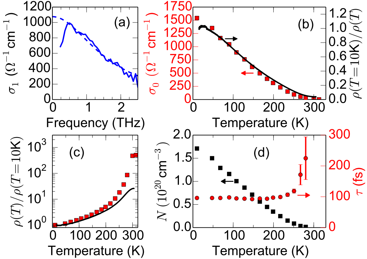
Figure 2: (a) Frequency-dependence of \sigma_1 for the VAN film at B = 0 and T = 86 K from experiment (solid line) and the Drude-Lorentz model (dashed line). (b) Temperature-dependence of \sigma_0 for the VAN film (squares, left axis) compared with the normalised dc conductivity \rho(T = 10 \text{ K})/\rho(T) (line, right axis). (c) THz resistivity normalized by resistivity at 10 K (squares, \sigma_0(10 \text{ K})/\sigma_0(T) ) compared with the ratio \rho(T)/\rho(T = 10 \text{ K}) for dc transport (line). (d) Mobile carrier density N (squares, left axis) and scattering time \tau (circles, right axis) for the VAN film, as a function of temperature.
