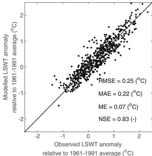
Fig. 4 Comparison of observed and modelled lake surface water temperature (LSWT) anomalies for 20 Central European lakes
