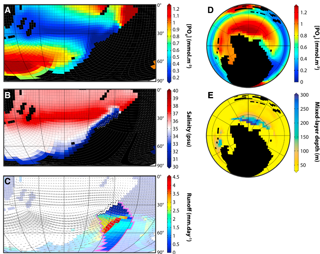
Figure 5. Analysis of the patterns of mean annual, surface phosphate concentration simulated using the 440 Ma continental land-sea mask and a solar forcing level of 350 \text{ W m}^{-2} . (a) \text{PO}_4 concentration in the Paleo-Tethys. (b) Ocean surface salinity in the Paleo-Tethys. (c) Near-surface winds (vectors) and continental runoff (shading) simulated in the same region. The pink contour delimits the watershed associated with the outlet constituted by the points highlighted with the dashed white line in Figure 5b, which correspond in turn to a zone of minimum of salinity. Grid points with no vectors are mountainous areas. Runoff here refers to the amount of water that is transferred from the continental grid points to the ocean (no routine scheme is implemented in this configuration of the model, see section 2.1.1). (d) South polar projection map of surface phosphate concentration. Laurentia is shown on top of the map. (e) South polar projection map of mixed-layer depth.
