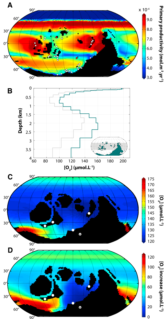
Figure 8. Impact of climate cooling on the primary productivity simulated at the ocean surface and on the oxygen concentration simulated throughout the water column. (a) Marine primary productivity simulated using the 440 Ma land-sea mask and a solar forcing level of 345 \text{ W m}^{-2} . White and red dots respectively stand for sediments of Hirnantian age associated with dysoxic-to-oxic and intermittently anoxic conditions (i.e., interbedded black shales), after the compilation of Melchin et al. [2013]. No continuous black shale deposition is reported during the Hirnantian. See Figure S2 for data points labeling. (b) Depth profiles of mean annual, tropical oxygen concentration simulated using the 440 Ma land-sea mask and solar forcing values of 350 \text{ W m}^{-2} (light grey curve) and 345 \text{ W m}^{-2} (dark grey curve). The insert in the bottom right corner represents the area over which data were averaged. The plot focuses on the tropical ocean, where major shifts in redox conditions are documented from the Katian to the Hirnantian [ Melchin et al. , 2013]. (c) Oxygen concentration simulated at the ocean bottom at 350 \text{ W m}^{-2} . (d) Increase in ocean bottom oxygen concentration simulated when decreasing solar forcing from 350 \text{ W m}^{-2} to 345 \text{ W m}^{-2} . Please note that the increase is positive everywhere. In Figures 8c and 8d, large white dots correspond to the location of the samples of Hammarlund et al. [2012], Zhang et al. [2009], and Yan et al. [2009]. The location of the well used by Vandenbroucke et al. [2015] is identified with a “W.”
