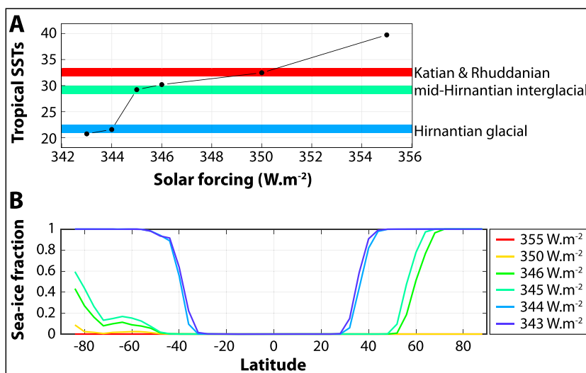
Figure 2. Climate results. (a) Mean annual tropical (30°S–30°N) sea surface temperatures as a function of the solar forcing level. We here represent the tropical sea surface temperatures (SSTs), instead of the global surface air temperatures, because Ordovician and Silurian isotopic data are gathered in locations situated at low paleolatitudes. As a consequence they exclusively report variations in tropical SSTs, which thus constitute the most straightforward variable for any model-data comparison [e.g., Trotter et al. , 2008; Finnegan et al. , 2011]. The colored strips identify the simulations selected throughout this study to investigate the mechanisms governing the deposition of black shales in the three time slices documented by Melchin et al. [2013]: the late Katian (red), the mid-Hirnantian (green), and the early Rhuddanian (red as well). The Hirnantian glacial state is shown for comparison (blue), but the associated model run is not analyzed in detail in this study. Please note that the colors of the strips correspond to the colors of the lines drawn in Figure 2b. (b) Mean annual latitudinal sea ice fraction simulated at various solar forcing levels.
