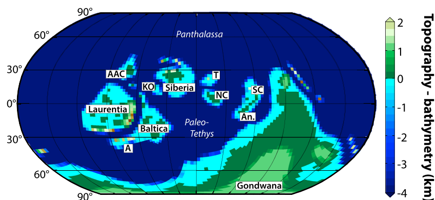
Figure 1. Late Ordovician-early Silurian continental reconstruction interpolated on the MITgcm cubed sphere grid: AAC: Arctic Alaska-Chukotka, KO: Kolyma-Omolon, A: Avalonia, T: Tarim, NC: North China, SC: South China, An: Annamia. Ocean names are in italic.
