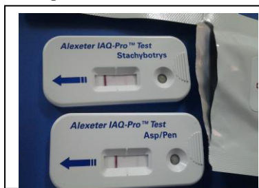
Figure 8: Result on IAQ MOLD Alexeter IAQ-Pro Asp/Pen® Test
