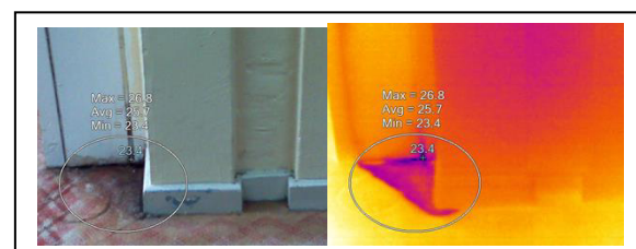
Figure 4: Infrared photo of carpet showing moisture intrusion from rain water down pipe
