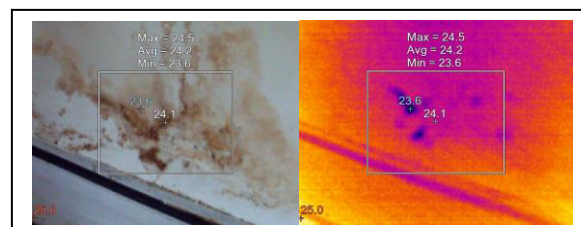
Figure 2: Infrared photo showing moisture intrusion into interior wall cavities
