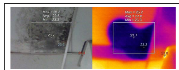
Figure 3: Infrared photo of ceiling showing moisture location
