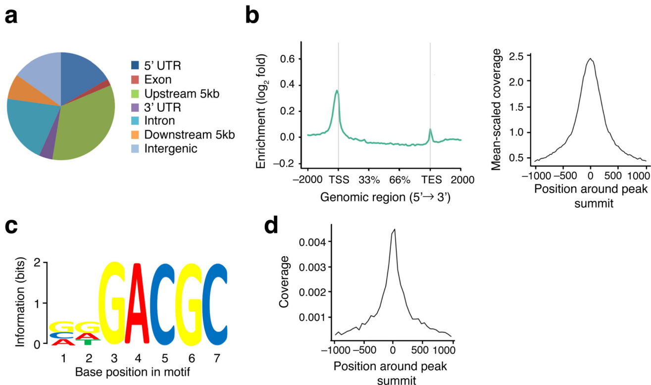
Figure 3. Foxn1 ChIP-seq analysis. (a) Proportion of Foxn1 ChIP-seq peaks falling within different RefSeq meta-gene regions. (b) Left: Enrichment of Foxn1 ChIP-seq signal across a meta-gene profile comprising all RefSeq mouse genes relative to control. TSS = transcriptional start site; TES = transcriptional end site. Right: Relative coverage of cTEC ATAC-seq transposon insertions relative to the summit of Foxn1 ChIP-seq peaks. (c) MEMEChIP-derived Foxn1 binding site motif for TSS-associated peaks (-5kb before and 100bp after TSS, E-value < 10^{-80} ). (d) Motif coverage relative to the summit of Foxn1 ChIP-seq peaks for TSS-associated peaks.
