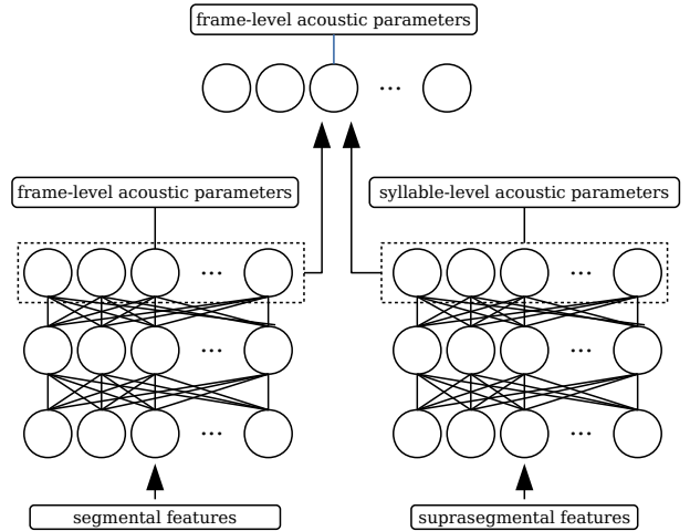
Figure 2: Hierarchical parallel deep neural network.
