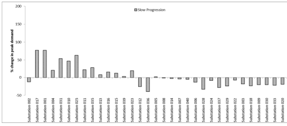
Figure 10: changes in winter peak demand relative to the base case for the Slow Progression scenario(substations with small floor area removed).
