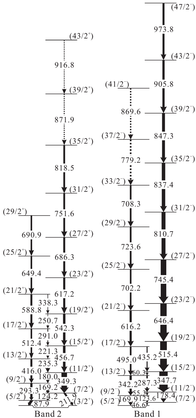
FIG. 3: Level scheme of ^{117}\text{Ba} proposed in this work.
