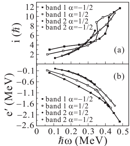
FIG. 6: (a) Extracted alignments and (b) Routhian energies for the ^{117}\text{Ba} rotational bands.
