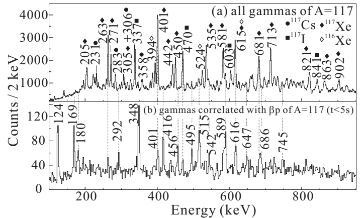
FIG. 2: Singles \gamma -ray spectra (a) gated on A = 117 residues and (b) tagged by \beta -delayed proton decay from A = 117 recoils within 5 s of implantation.
