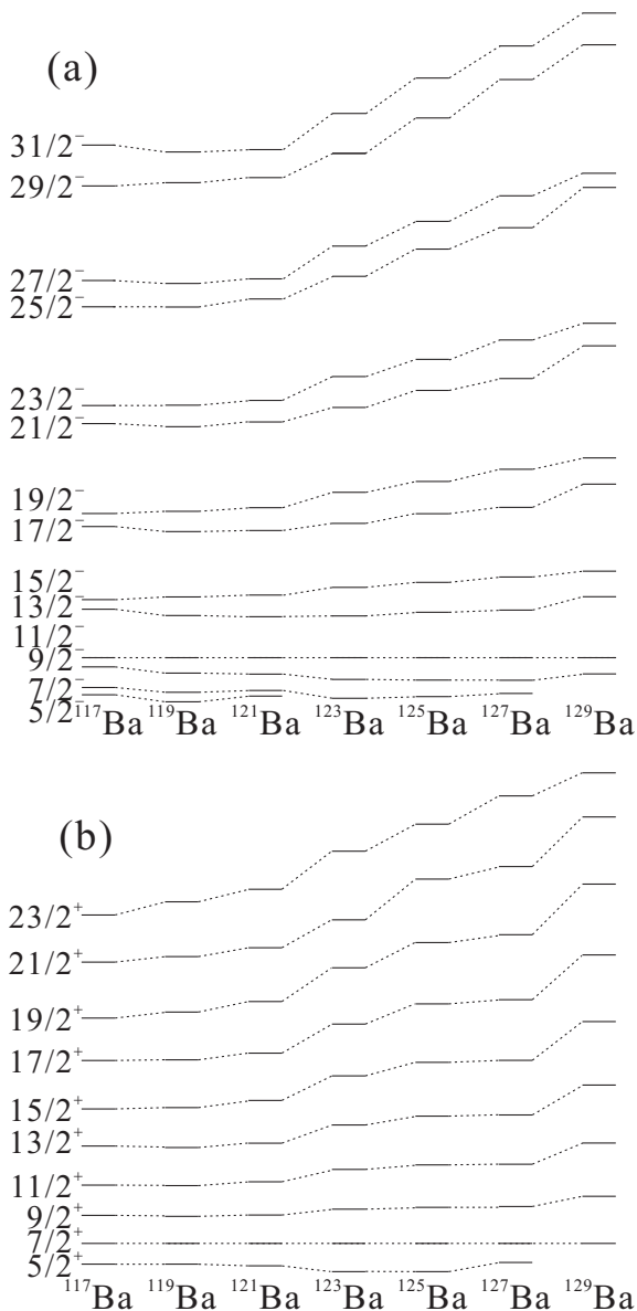
FIG. 5: Level-spacing systematics for (a) negative- and (b) positive-parity bands in the odd-A ^{117-129}\text{Ba} isotopes. The energies are normalized to the respective 11/2^- ( 7/2^+ ) states of negative-parity (positive-parity) bands. The data are from Refs. [8, 9, 17, 18, 35, 36] and the present work.
