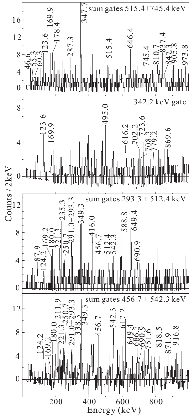
FIG. 4: Representative coincidence spectra with gates placed on selected transitions in bands 1 and 2.
