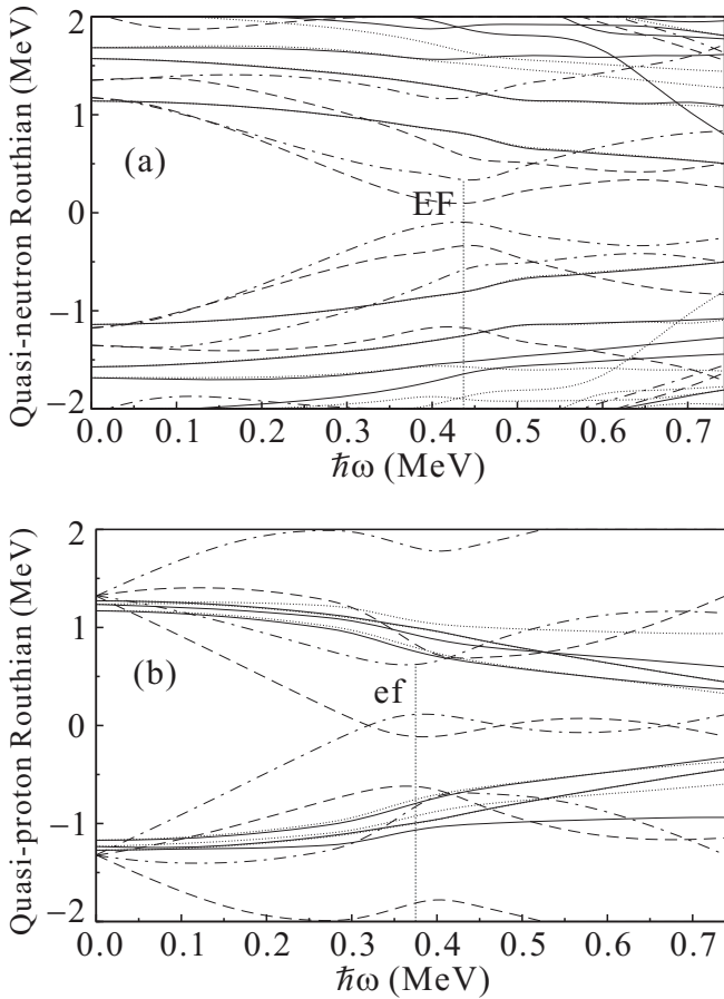
FIG. 7: Calculated quasiparticle Routhians for (a) neutrons and (b) protons as a function of rotational frequency ( \hbar\omega ). The deformation used in the calculations are give in the text. The different line styles represent values of parity and signature, (\pi, \alpha) , as follows: dashed lines (-, -1/2) ; dot-dashed lines (-, +1/2) ; solid lines (+, +1/2) ; and dotted lines (+, -1/2) . The lowest neutron and proton Routhians with \alpha = +1/2 and \alpha = -1/2 are both the h_{11/2} orbitals. The positions of the lowest alignments for neutrons, e.g., EF in panel (a) and protons, e.g., ef in panel (b) are marked by faint vertical dotted lines.
