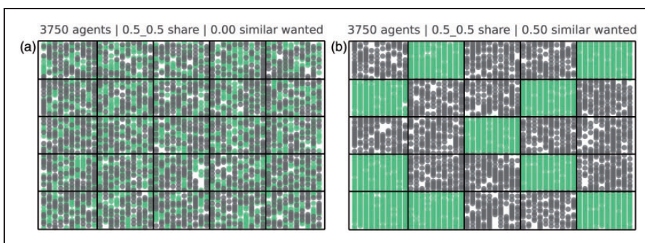
Figure 1. Output map examples (two groups): (a) \tau = 0 and (b) \tau = 0.5 .
