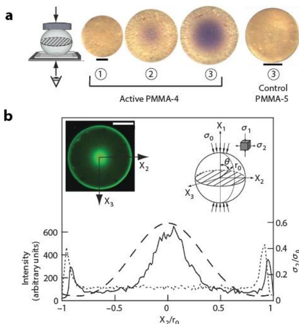
Figure 14. a) Compression of beads of glassy crosslinked spirocyan derivative PMMA (called “Active PMMA-4” in the figure) yields color and fluorescence with spatial distribution of intensity (solid line in b) consistent with the calculated distribution of normalized traverse stress (dashed line in b). Reprinted with permission from ref. [188]. Copyright © 2009, Rights Managed by Nature Publishing Group.
