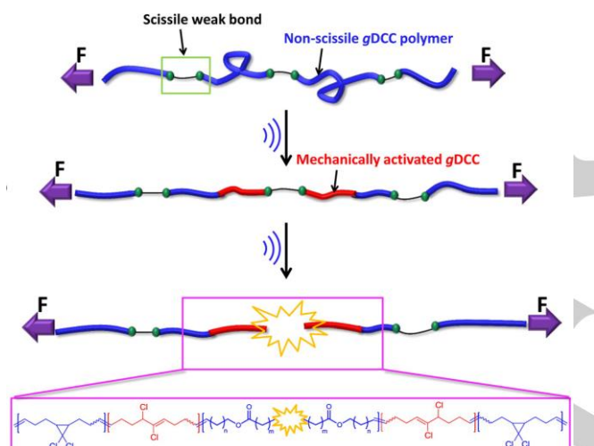
Figure 11. Sonication of polymers containing cyclopropane moieties (gDCC, blue) and weak bonds (S-C, C-O or N=N, green) in the backbone leads to isomerization of cyclopropane moieties to olefins (red) and fragmentation of the polymer. Adapted from ref [97] under Creative Commons License.
