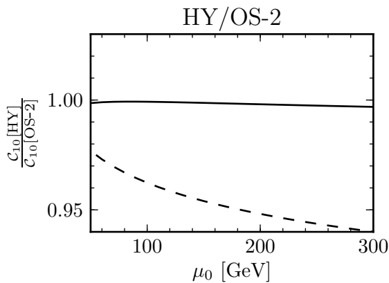
FIG. 4. The \mu_0 dependence of the ratio of the Wilson coefficient \mathcal{C}_{10}(\mu_b = 5 \text{ GeV}) in the HY and the OS-2 scheme at LO and NLO QCD (dashed) and NLO (QCD + EW) (solid). LO and NLO QCD curves coincide.
