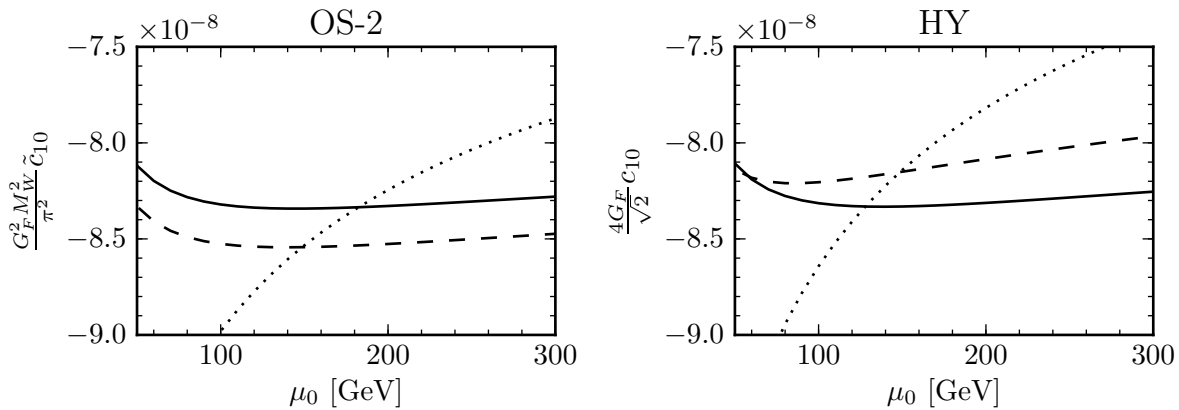
FIG. 3. The \mu_0 dependence of the Wilson coefficient \mathcal{C}_{10}(\mu_b = 5 \text{ GeV}) in two renormalization schemes (OS-2, HY) at LO (dotted), NLO QCD (dashed) and NLO (QCD + EW) (solid). See text for more details.
