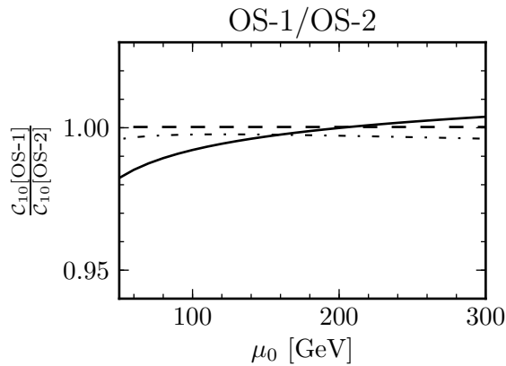
FIG. 6. The \mu_0 dependence of the ratio of the Wilson coefficient C_{10}(\mu_b = 5 \text{ GeV}) in OS-1 and OS-2 schemes. The LO and NLO QCD result coincide (dashed). The full \mu_0 dependence of NLO (QCD + EW) (solid) and partial \mu_0 dependence for fixed m_t(160 \text{ GeV}) in the s_W -on-shell counterterm (dashed dotted).
