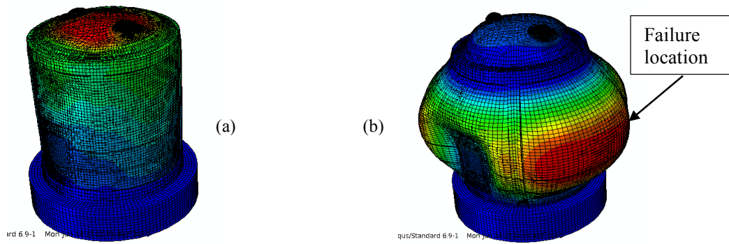
Figure 2. Predicted response of the BARC model (a) under prestress only and (b) at P=2.89 P_d
