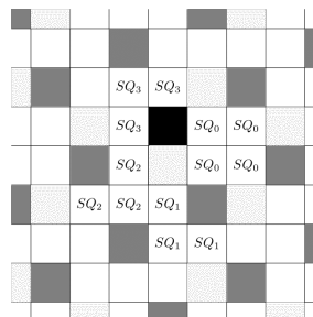
Figure 4: Attack on SQ_3
