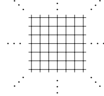
Figure 1: The Infinite Grid G_\infty
