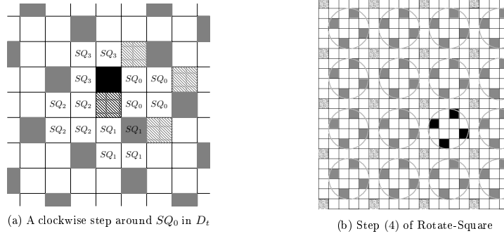
Figure 3: Steps (3) and (4) of Rotate-Square
