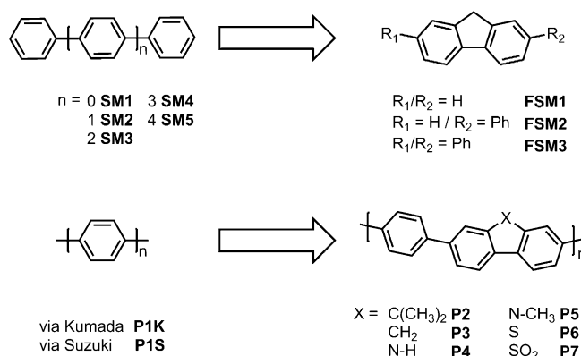
Figure 1. Structures of conjugated phenylene oligomers (SM1–SM5) and poly( p -phenylene)s (P1K, P1S; left) and their planarized fluorene-tylone analogs (FSM1–FSM3, P2–P7; right).
