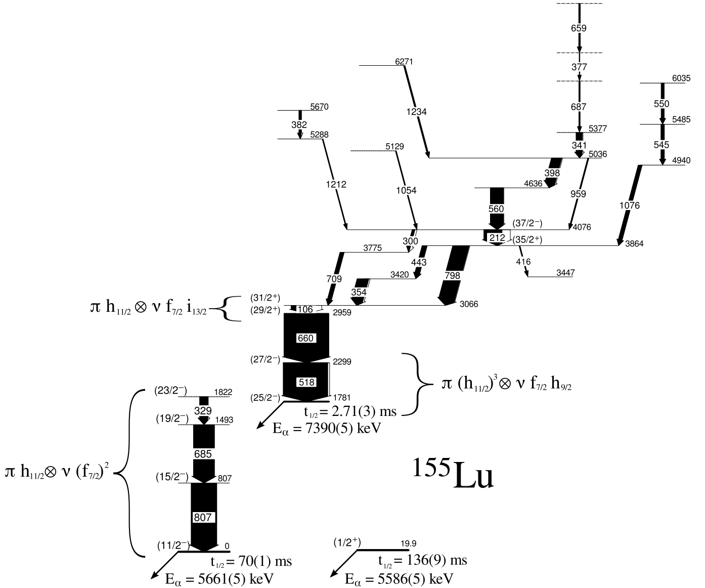
FIG. 3: Revised and extended level scheme of excited states in ^{155}\text{Lu} . Energies are in units of keV.
