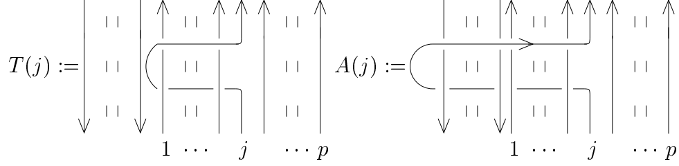
FIGURE 14. The tangles representing the elements T(j) and A(j) for 1 \leq j \leq p .
