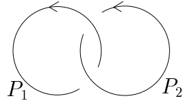
FIGURE 2. The link H_+(P_1, P_2) .
