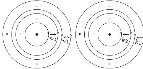
FIGURE 3. The diagrams P_1 and P_2 .
