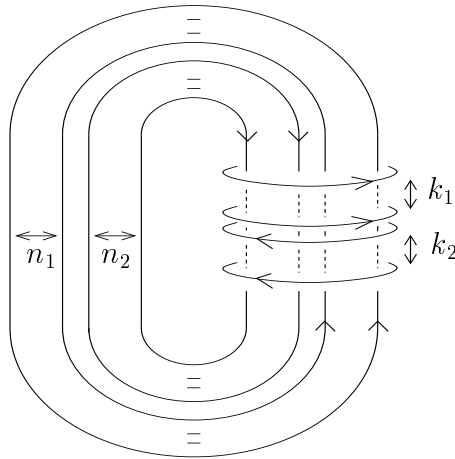
FIGURE 4. The generalized Hopf link H(k_1, k_2; n_1, n_2) .
