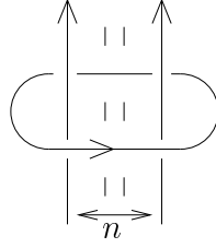
FIGURE 9. The n -tangle T^{(n)} .
