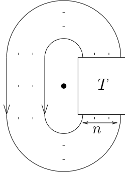
FIGURE 8. An element of the subspace \mathcal{C}^{(n)} .
