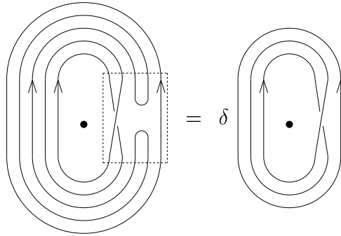
FIGURE 11. The generator A_{-2}A_1 .
