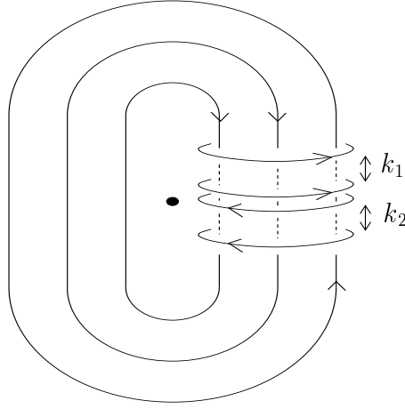
FIGURE 15. The link H(k_1, k_2; 1, 2) in \mathcal{C} .
