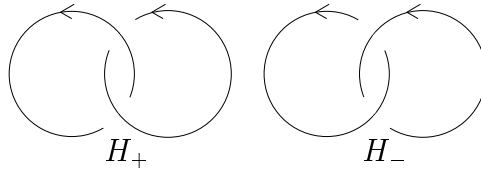
FIGURE 1. The links H_+ and H_- .
