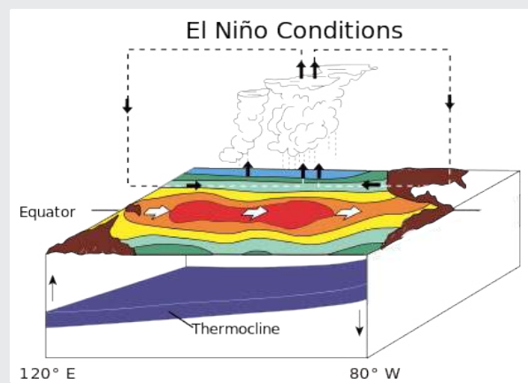
Warm conditions extend all the way across the Pacific with the sea surface sloping upwards from west to east and the thermocline flattening off, sinking in the east and restricting upwelling. The Focus of the Walker Circulation moves to over the central Pacific resulting in westward flowing surface winds flowing across half the Pacific reducing the intensity of the easterlies.
