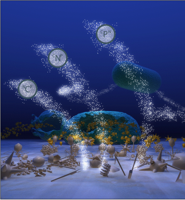
Figure 3.1.3 The death of microbial cells releases an important source of elements (C, N and P) that play a pivotal role in global biogeochemical cycles. (Graphic Michael Tangherlini).
