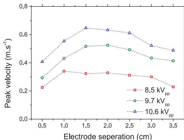
Figure 5. Peak velocity measured downstream of a single electrode pair as a function of electrode separation, at applied voltages of (triangles) 10.6 \text{ kV}_{pp} , (circles) 9.7 \text{ kV}_{pp} (squares) 8.5 \text{ kV}_{pp} .
