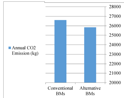
Fig.8.Comparison of annual CO2 emissions
