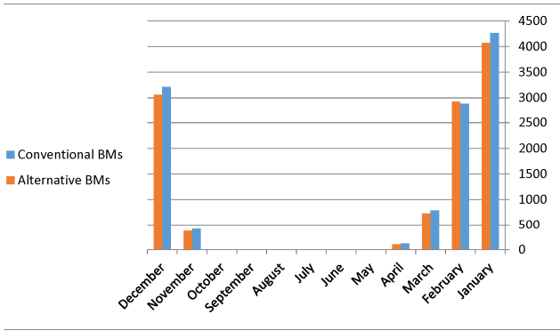
Fig.5.Comparison of monthly thermal energy consumption
