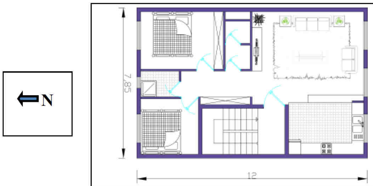
Fig.2. Typical floor plan of the case study
