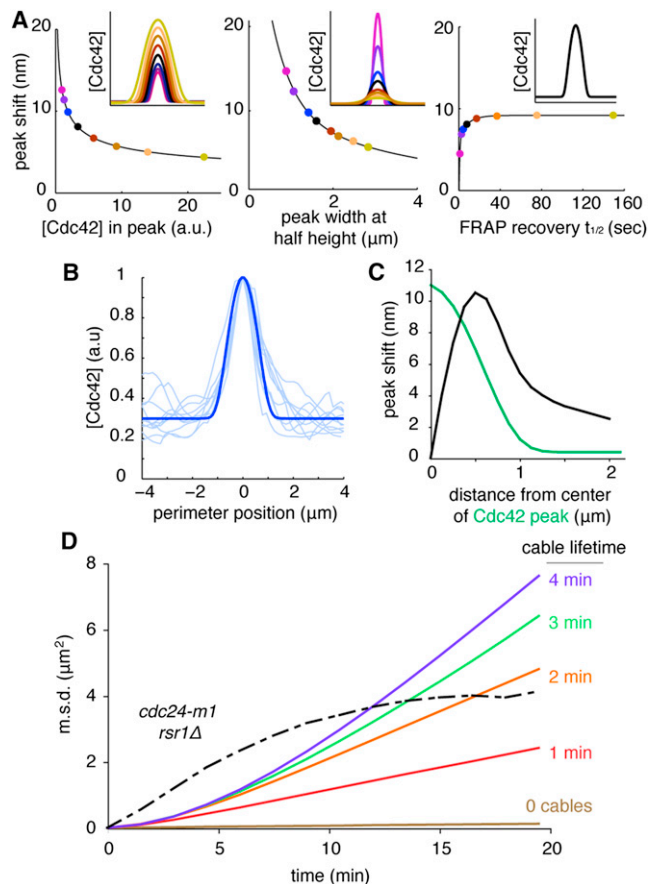
Figure 4. Simulated Wandering due to Vesicle Traffic
