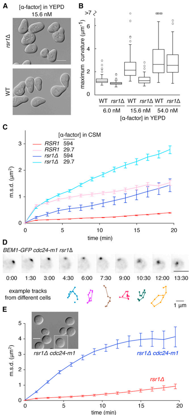
Figure 2. Wandering Is Constrained by Rsr1 and by Gβγ-Far1 at High Pheromone Concentration
