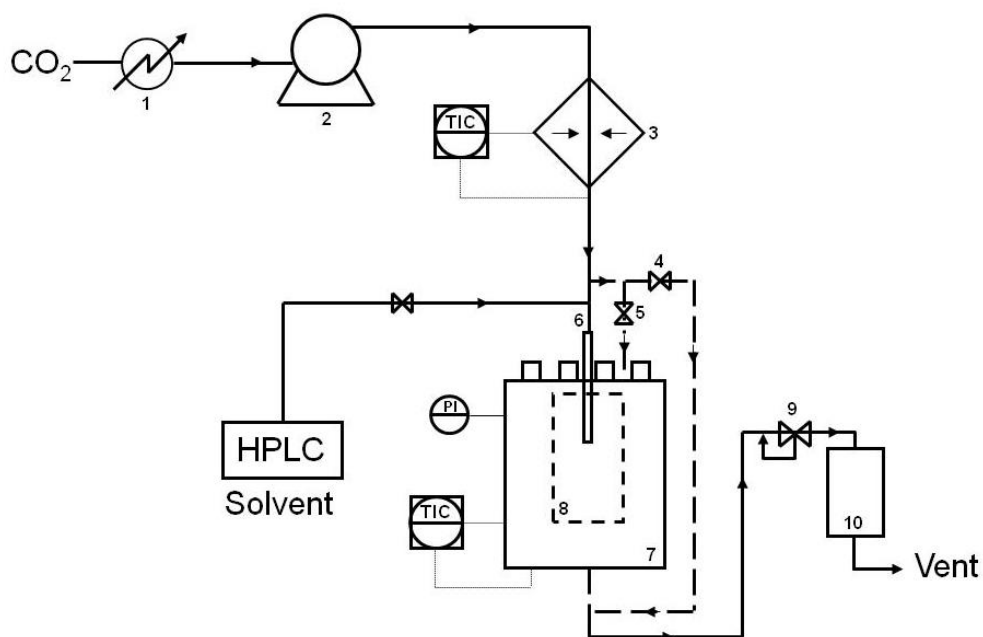
Figure 1. Technical diagram of Separex SAS equipment. (1) Chiller; (2) liquid pump; (3) heat exchanger; (4) and (5) by-pass valves, (6) co-axial nozzle for CO 2 and metal salt solution delivery; (7) precipitation vessel; (8) sample recovery vessel; (9) back pressure regulator and (10) separation vessel.
