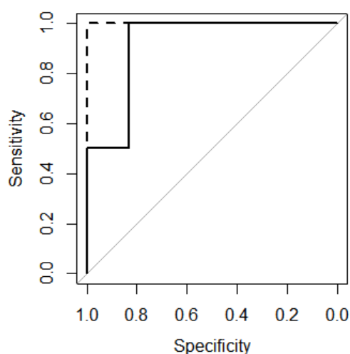
Figure 3. ROC curves for the SVM (—), RF (---) and NN (.....) models (RF and NN plots lie on top of each other)
