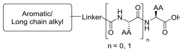
Figure 1. Generic structure of library (AA – amino acid); see Supporting Information for specific structures.
