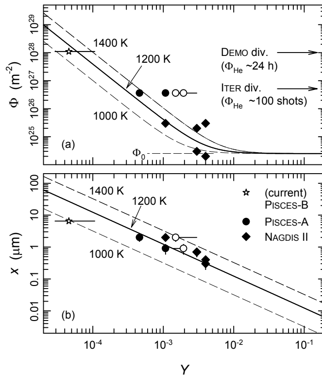
Figure 5. Plot of (a) \Phi_{\text{eq}} and (b) x_{\text{eq}} , as a function of erosion yield Y , produced from equations (10) and (11). Full and dashed lines correspond to adjusted C values corresponding to 1000, 1200, and 1400 K, using the temperature dependence in [1]. Overlaid data points are fuzz layer thicknesses corresponding to the erosion regimes and references of table 2. Open symbols pertain to cases with measured fuzz yields and to compare to line plots Y_{\text{fuzz}}/(1-p) is used for the abscissa. Similarly, full symbols are those of bulk yields. To compare these the abscissa is Y_{\text{bulk}}/5 . See table 2 footnotes.
