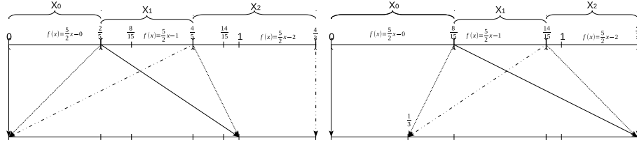
Fig. 2. Deterministic greedy (on the left) and lazy (on the right) \frac{5}{2} -expansion PAM
