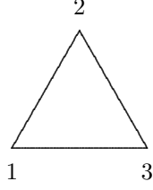
Figure 1: Winding Number and (1, 2, 3)-Triangle
